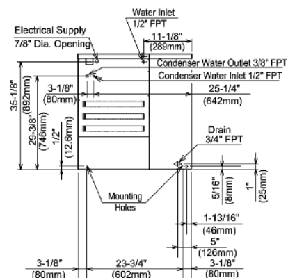
WATER-COOLED UNIT
